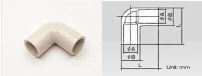
NDE-20, 90 astetta
